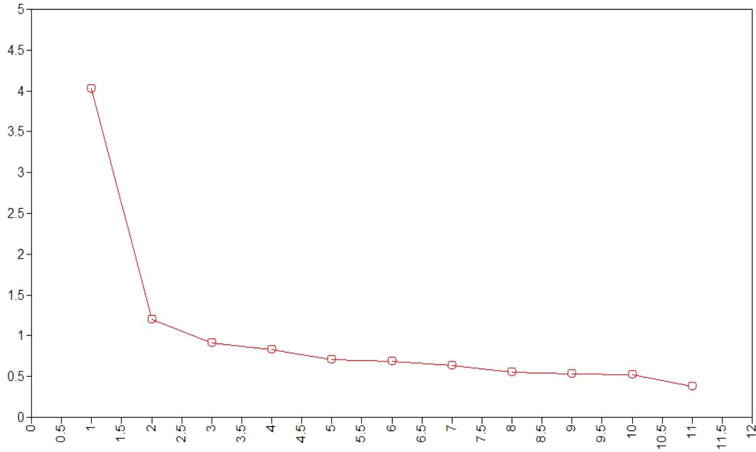
Figure 1: Scree plot Part I
