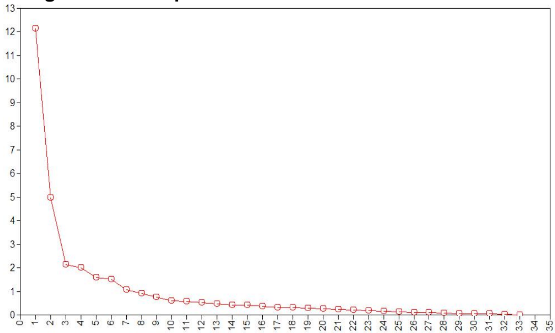
Figure 4: Scree plot for Part IV
