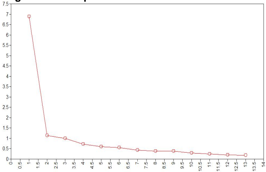
Figure 2: Scree plot Part II
